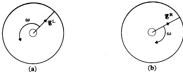
4.2 In circularly polarised radiation the electric field vectors \mathcal{E}^L , and \mathcal{E}^R rotate in anticlockwise and clockwise directions when facing into the oncoming wave.
